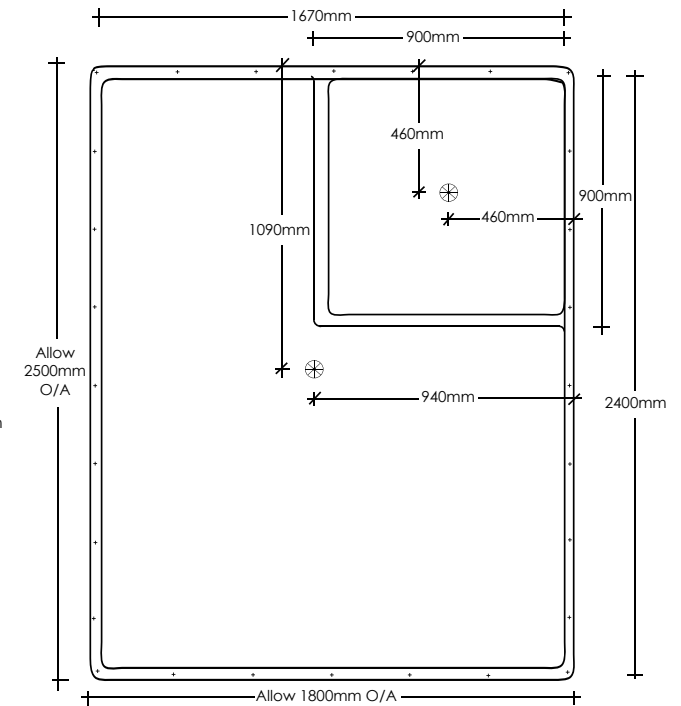
FLOOR PLAN
