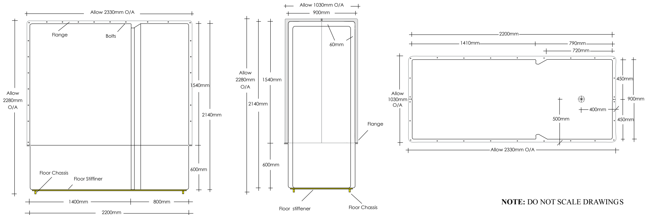
FLOOR PLAN
