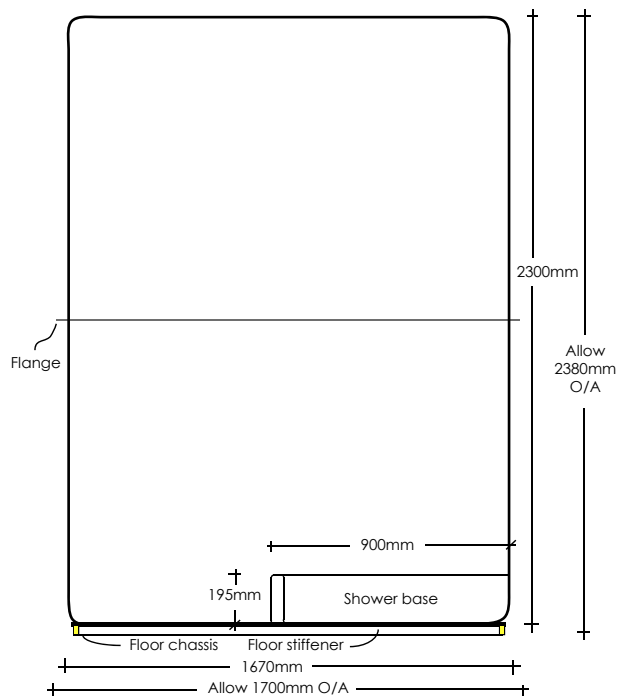
END / SIDE ELEVATION
